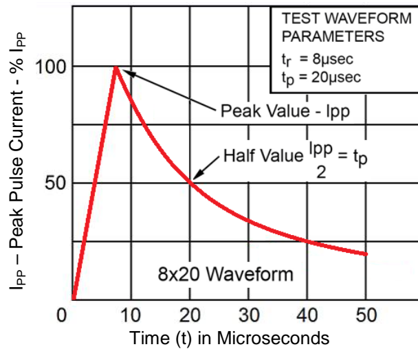
FIGURE 3 8/20 μs Current Impulse Waveform
